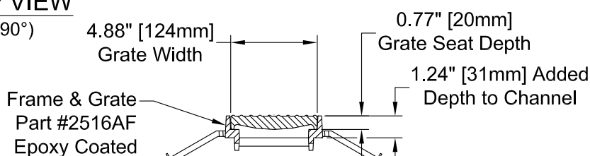
GRATE END VIEW
