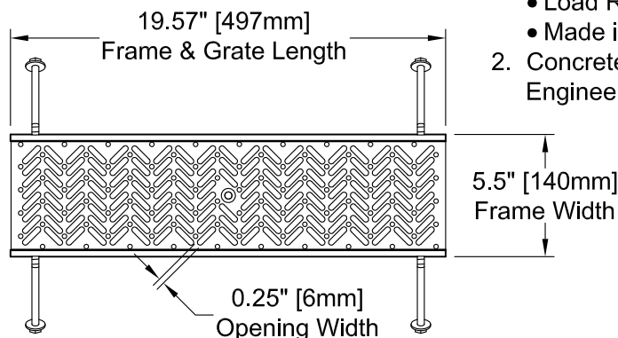
GRATE TOP VIEW
